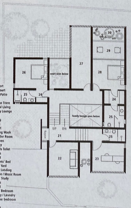
First Floor Plan N 0 2 5 10 ft
