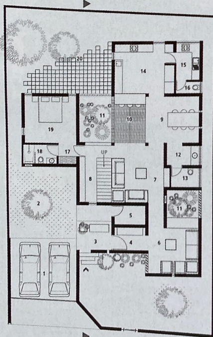
Ground Floor Plan N 0 2 5 10 ft
